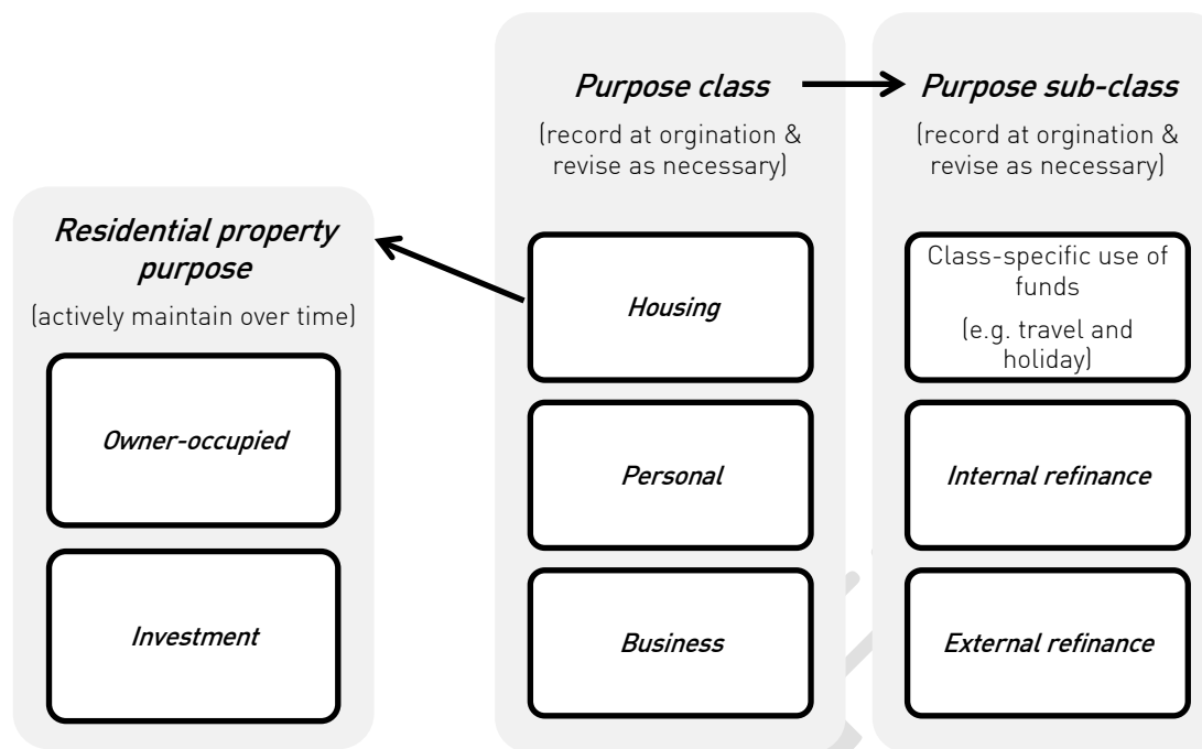
Figure 4: Purpose Types
